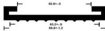
REF. ZUNCHO 2 - 1/2 ROLLO X 50 MTS.
