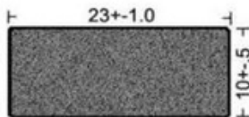
REF. ZT - 13 = TIC - 100 AJUSTE CAPOT VARIOS ROLLO X 50 MTS
