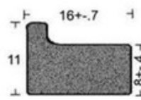
REF. T - 17 = TIC - 72 PUERTA MERCURI Y NISSAN ROLLO X 50 MTS
